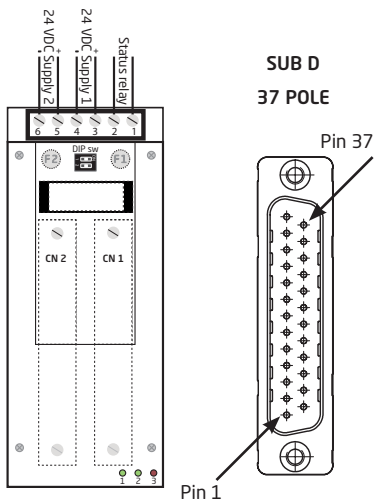
BACKPLANE DUAL CONNECTORS
